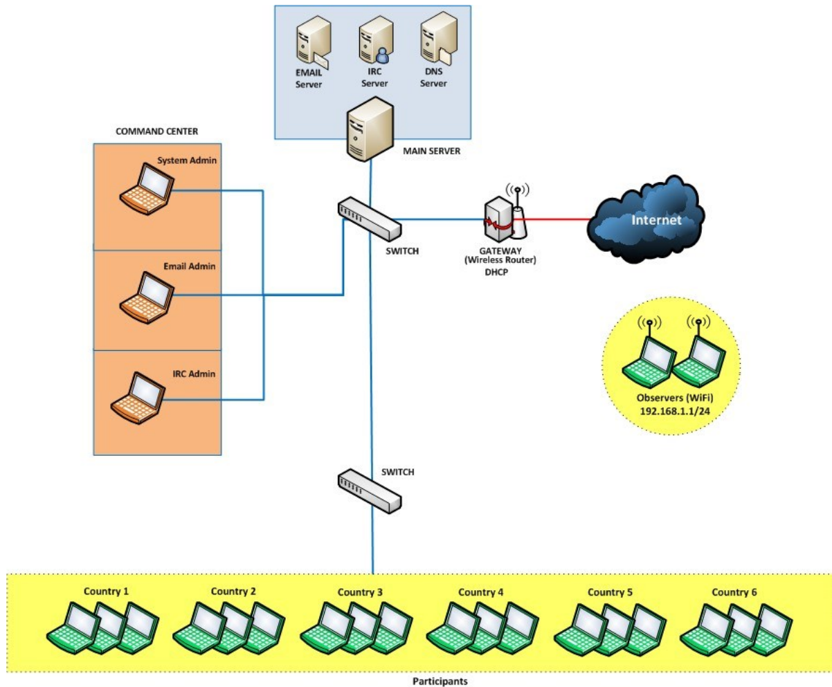
Figure 3 : Drill Setup
