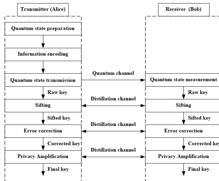
Figure 8 – Flowchart of decoy-state BB84 protocol
