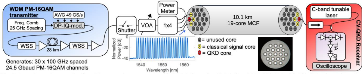
Figure 18 – Experimental schematic of the effect of crosstalk between cores in a multicore fibre on the CV-QKD system
