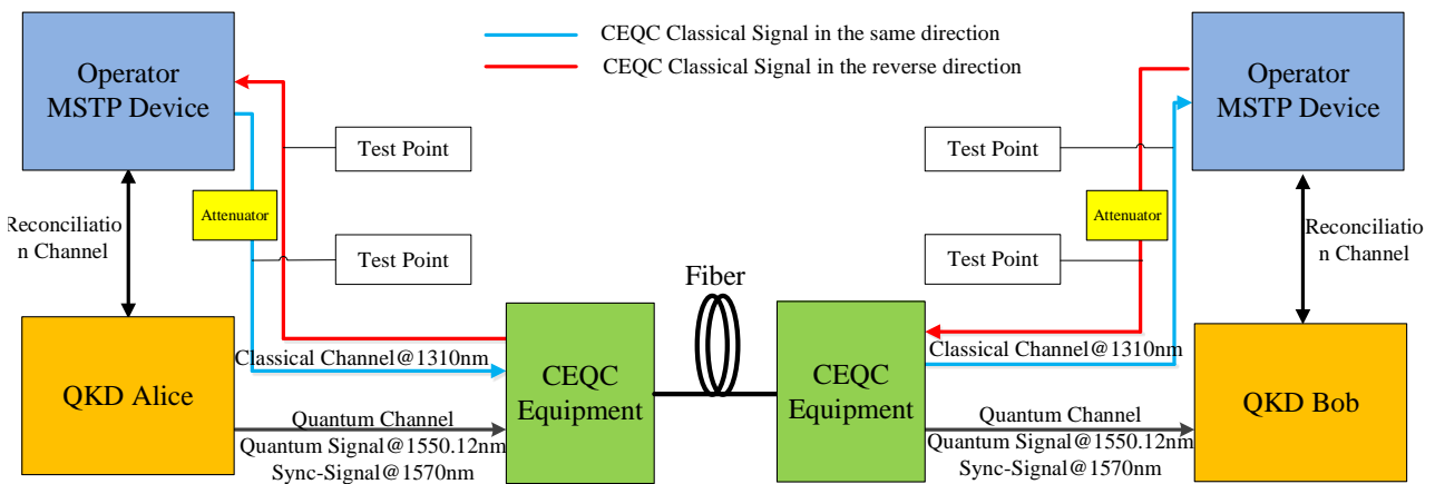
Figure 25 – Experimental system of CEQC based on grey light communication
