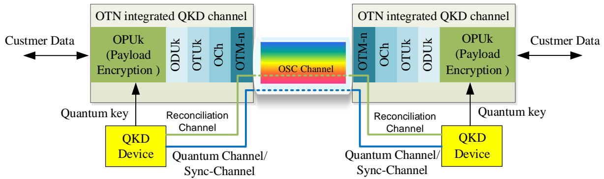
Figure 21 – CEQC between QKD and OTN system
