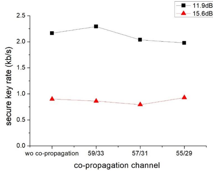
Figure I.11 – Secure secret key rate over different channel space between CV-QKD and classical signal
