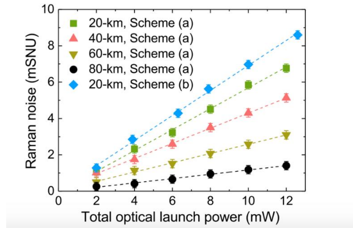
Figure 14 – Relationship between optical launch power and Raman noise
