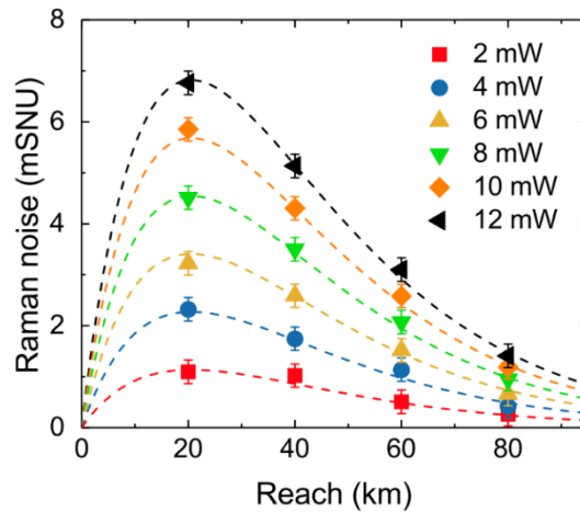
Figure 15 – Relationship between transmission distance and Raman noise
