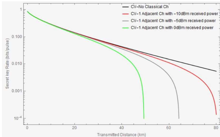
Figure I.6 – Secure secret key rate of CV-QKD system under different classical optical power
