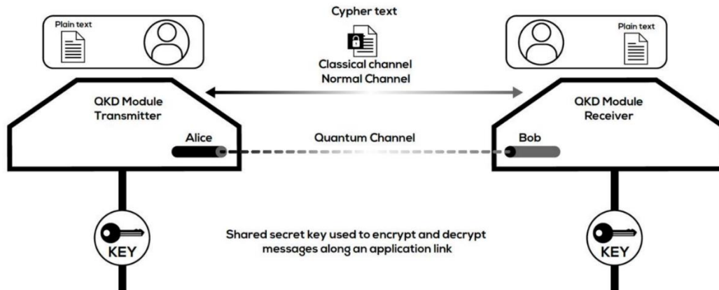
Figure 1 – Point-to-point QKD link
