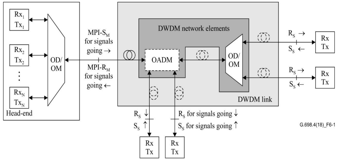
Figure 27 – G.698.4 system model
