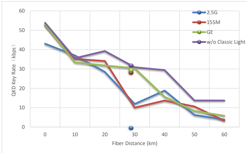
Figure I.7 – QKD key rates figure based on MSTP system and 40M Polarization coding QKD with the same direction
