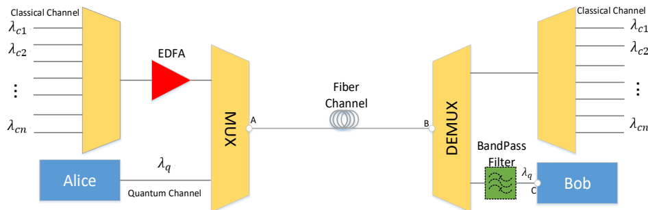
Figure 24 – Typical schematic of CEQC of classical optical and QKD quantum signal
