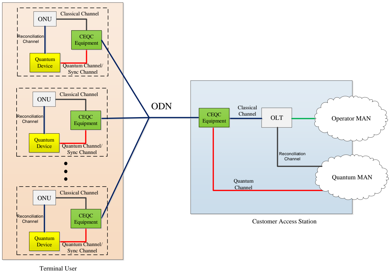
Figure 23 – CEQC Scheme for PON access users
