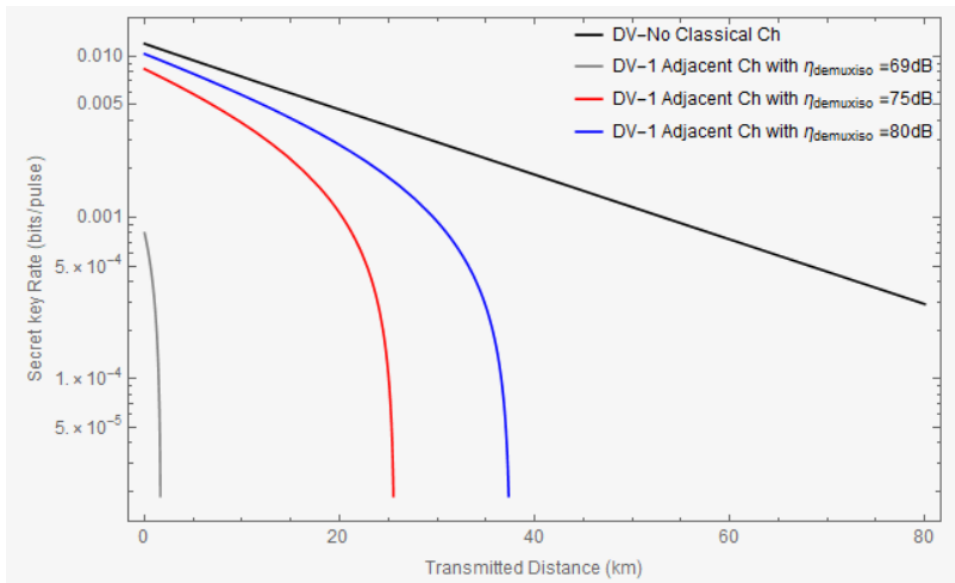
Figure I.1 – Impact of channel isolation on secure secret key rate of DV-QKD System
