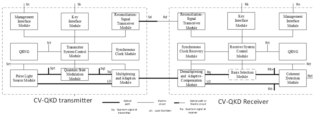
Figure 11 – Reference points for the CV-QKD system
