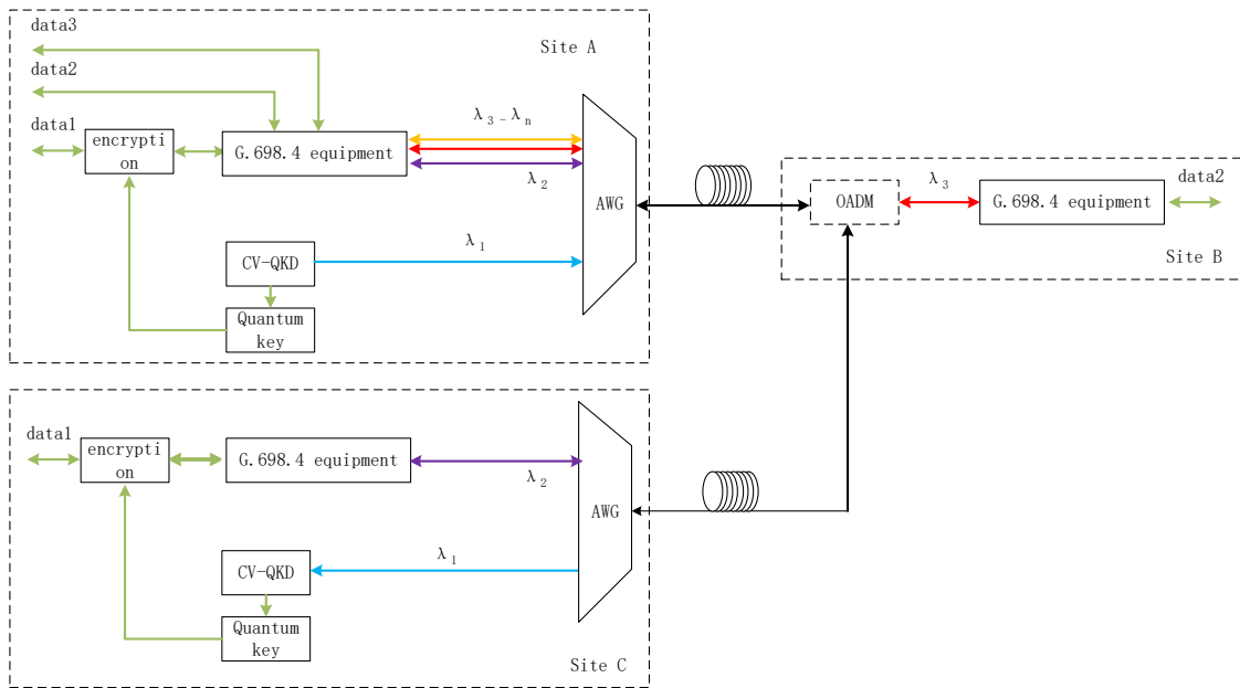
Figure 28 – Network scheme based on CV-QKD and G.698.4 system
