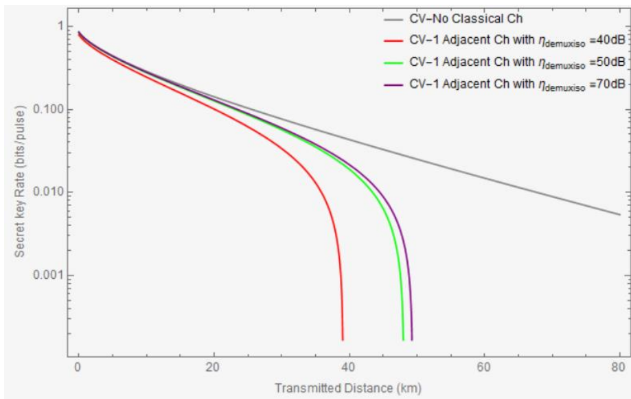
Figure I.2 – Impact of channel isolation on secure secret key rate of CV-QKD System
