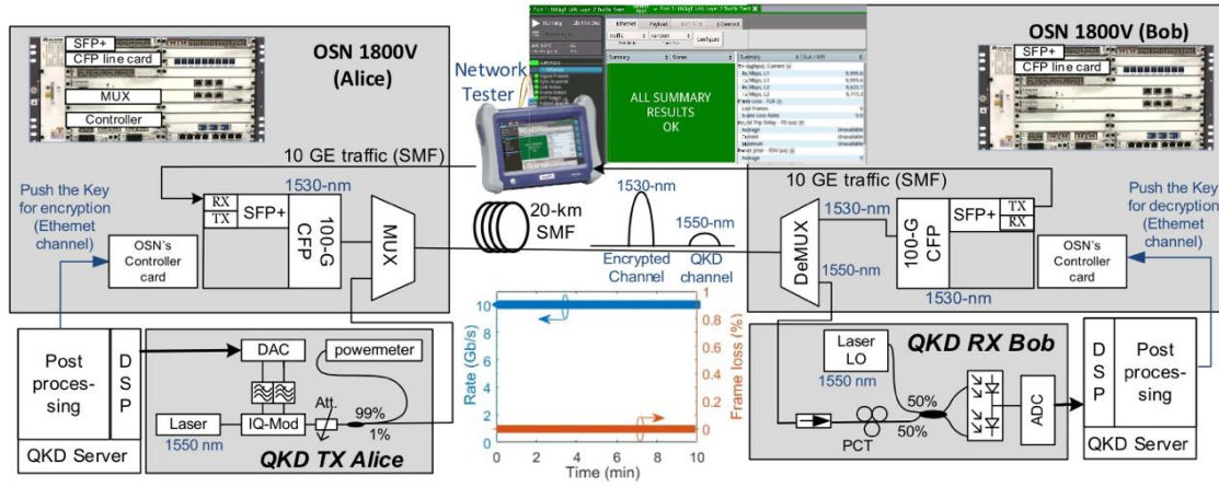
Figure 16 – Application of CV-QKD to OTN networks for real-time encryption experiments on 10GE services [b-Karinou]
