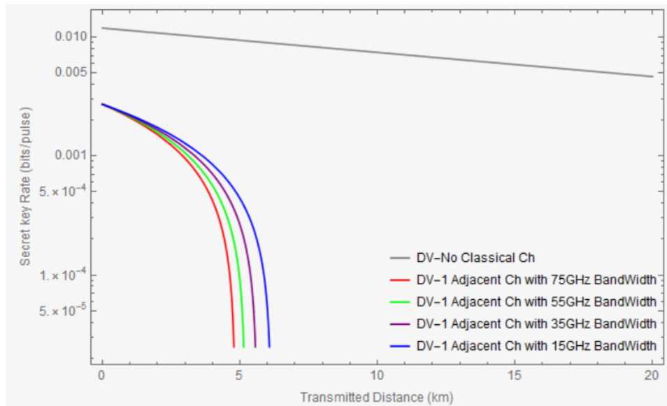
Figure I.4 – Impact of quantum channel bandwidth on secure secret key rate of DV-QKD system
