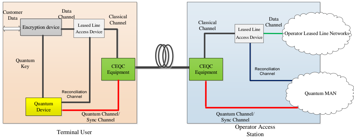
Figure 22 – CEQC access scheme to operator network
