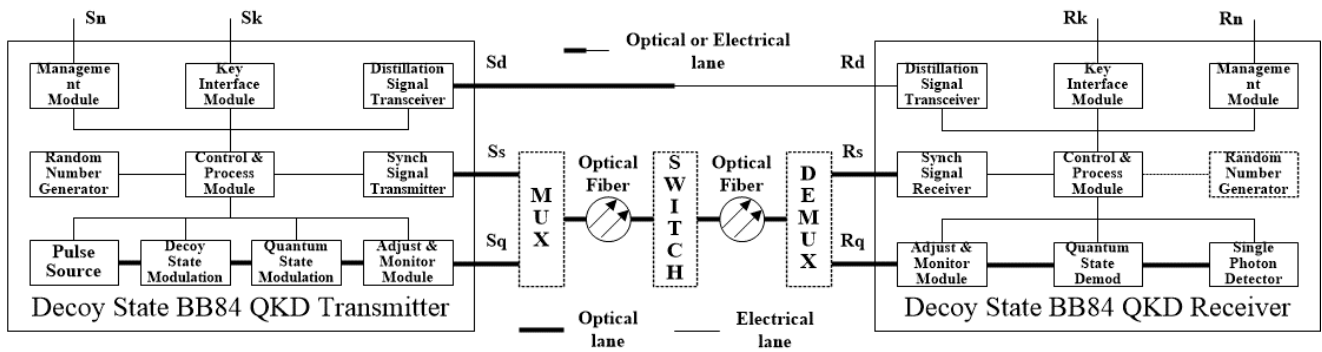
Figure 9 – System model and reference points of decoy-state BB84 system
