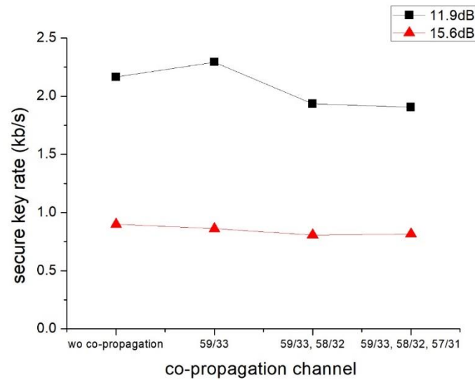
Figure I.12 – Secure key rate over different channel amount of classical signal
