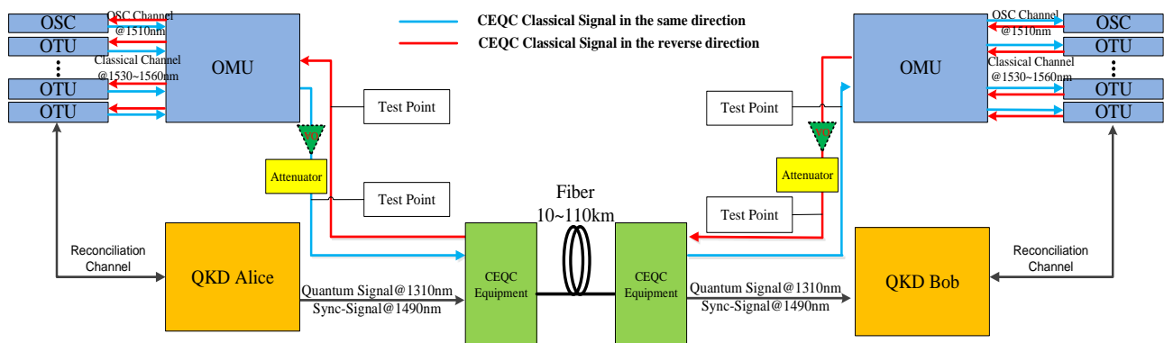
Figure 26 – CEQC test system based on WDM system
