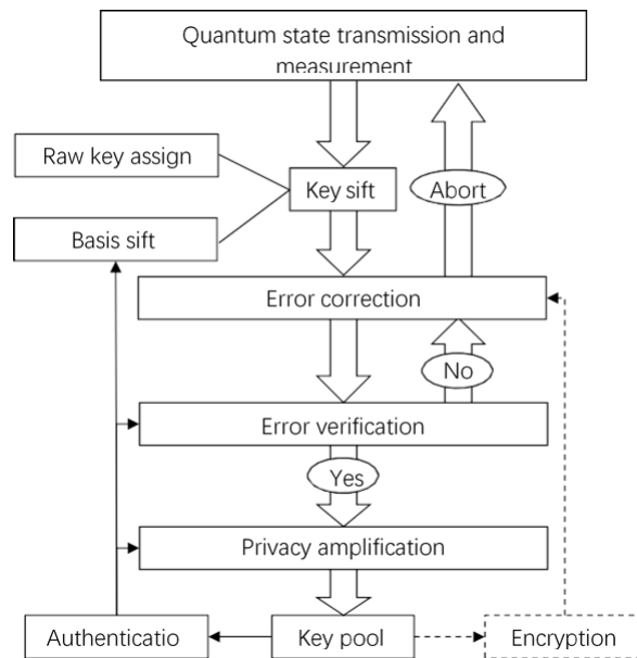
Figure 10 – Flowchart of data postprocessing procedures [b-Xu]
