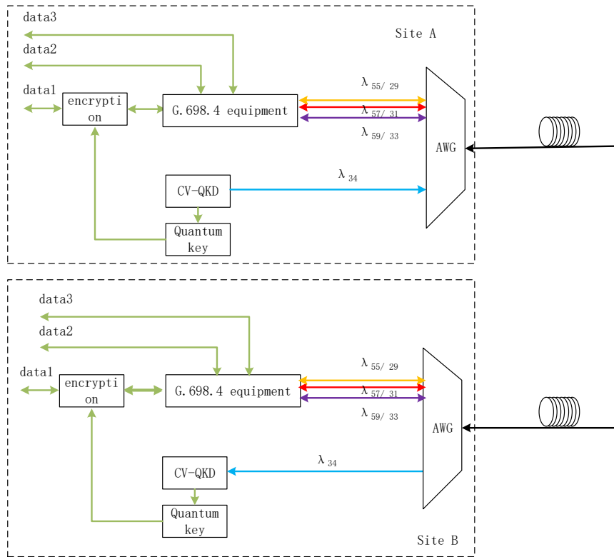
Figure I.10 – Experiment setup
