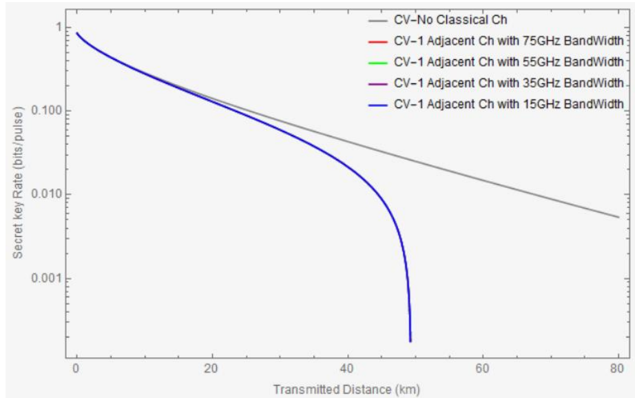
Figure I.3 – Impact of quantum channel bandwidth on secure secret key rate of CV-QKD system
