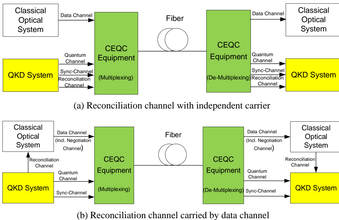
Figure 20 – Combination of QKD network and existing optical fibre system
