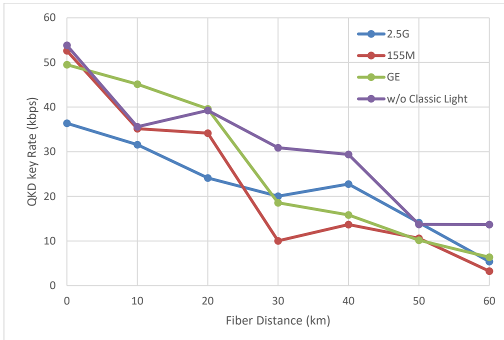
Figure I.8 – QKD key rates figure based on MSTP system and 40M polarization coding QKD with the contrary direction
