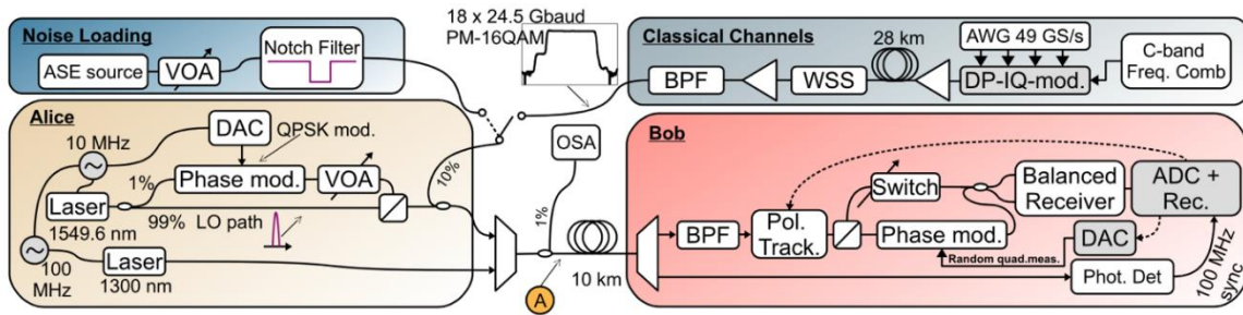
Figure 17 – Experimental scheme in [b-Eriksson-1]
