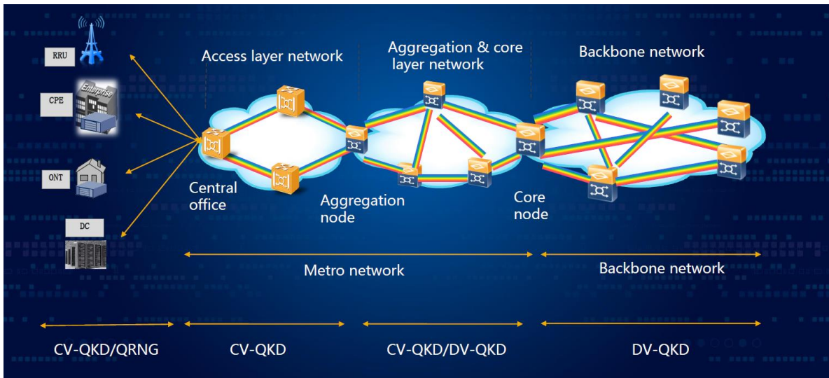
Figure 4 – Optical network with QKD [b-Zhao]
