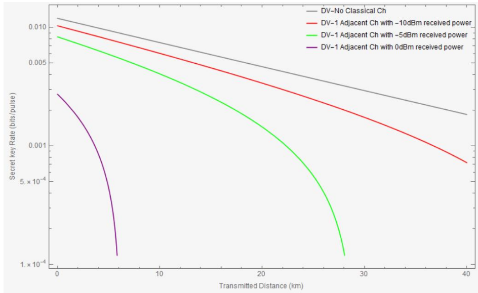
Figure I.5 – Secure secret key rate of DV-QKD system under different classical optical power
