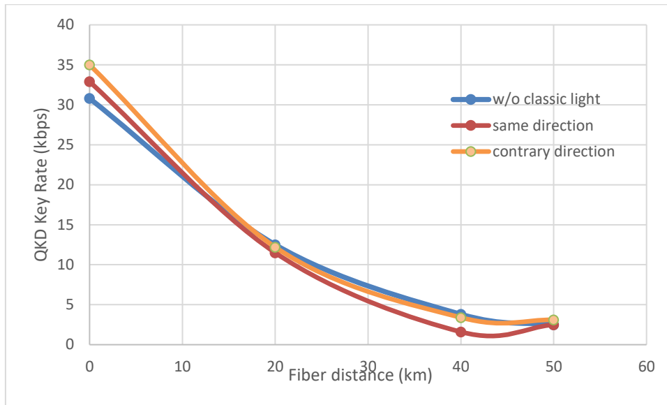
Figure I.9 – QKD key rates figure based on WDM system and GHz polarization coding QKD
