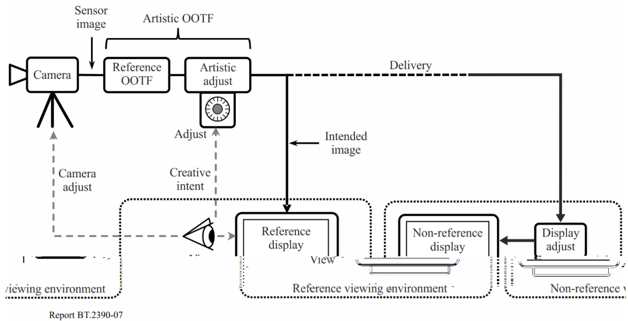
FIGURE 7 The conceptual TV system
